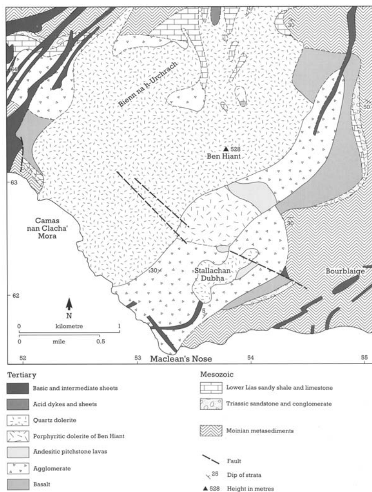
Figure 4.2: Geological map of the Ben Hiant site (after Gribble, 1976)
