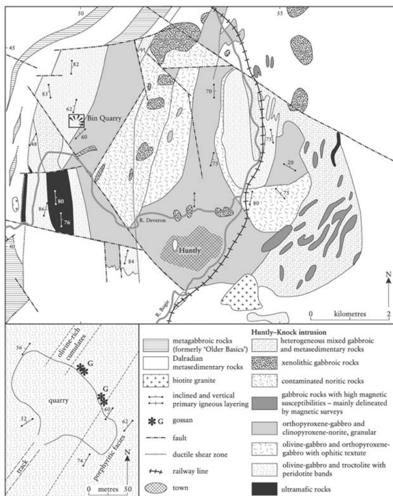
Figure 3.6: Map of the southern part of the Huntly–Knock intrusion, from BGS 1:50 000 Sheet 86W (in press), with details of the Bin Quarry GCR site, from Gunn and Shaw (1992).
