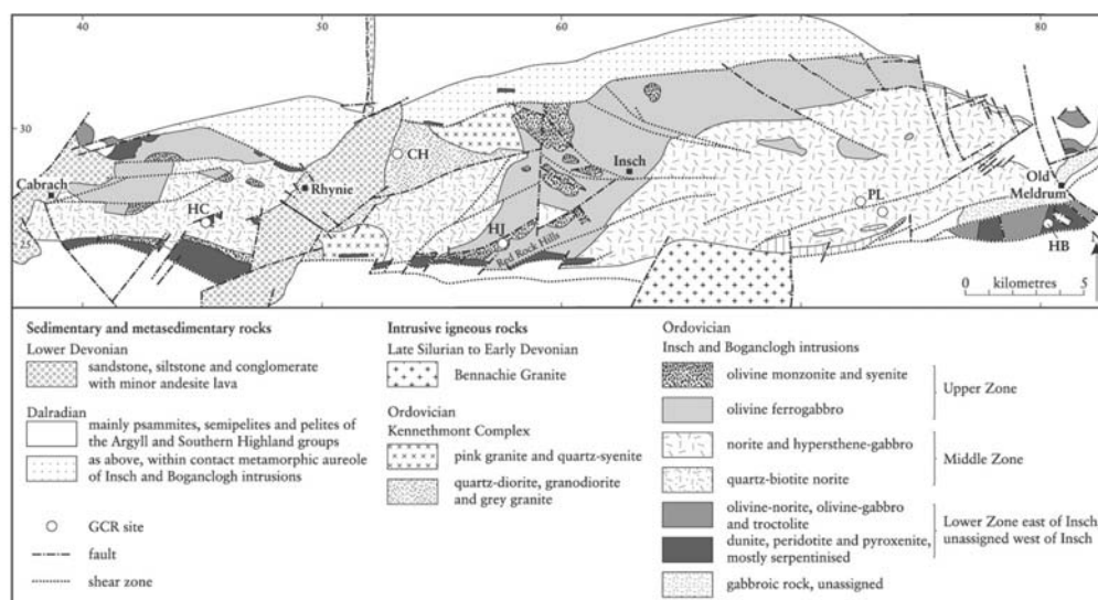
Figure 3.2: Map of the Insch, Boganclogh and Kennethmont intrusions, adapted from Gould (1997). GCR sites: CH Craig Hall; HB Hill of Barra; HC Hill of Craigdearg; HJ Hill of Johnston; PL Pitscurry and Legatesden quarries.
