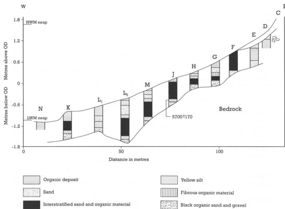
Figure 12.9: Profile across the intertidal deposits at Borve, showing the sediment sequence and its variations (from Ritchie, 1985).
