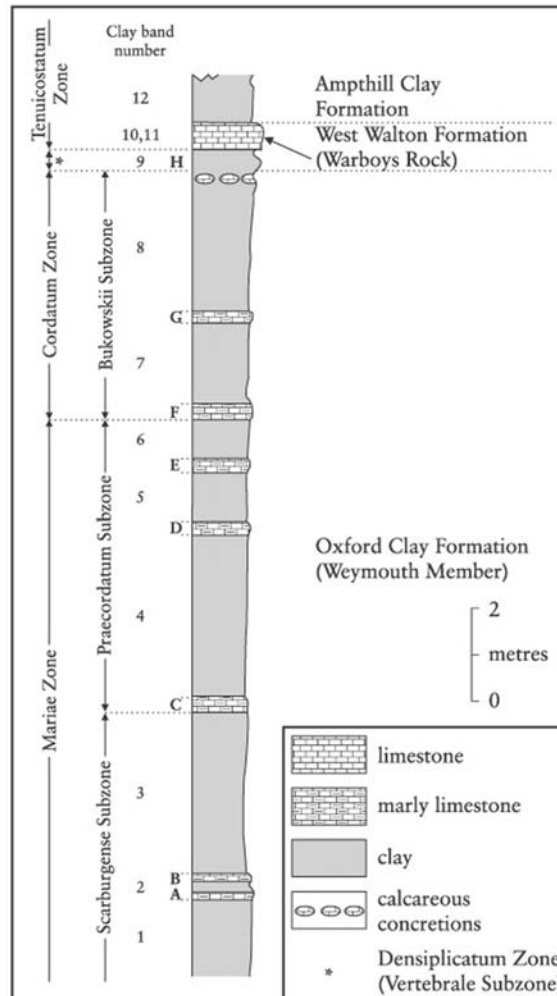
Figure 3.6: Log of the Oxford Clay succession in Warboys Pit (after Callomon, 1968).
