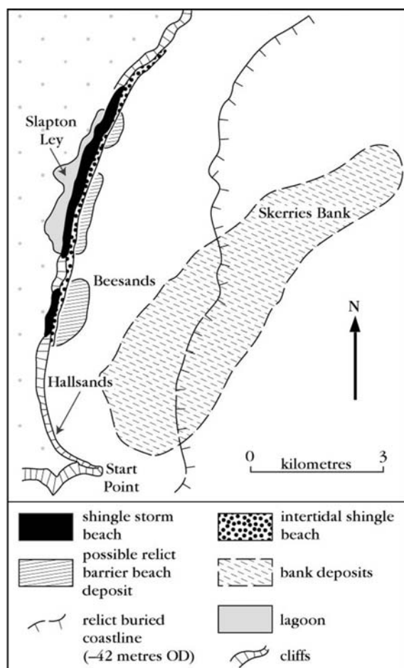
Figure 6.6: Hallsands and Slapton Sands represent parts of a once-continuous gravel beach. Offshore, there is evidence of buried shorelines and a possible former barrier beach. The present-day shingle beach is separated by rock headlands. (After Hails, 1975a.)
