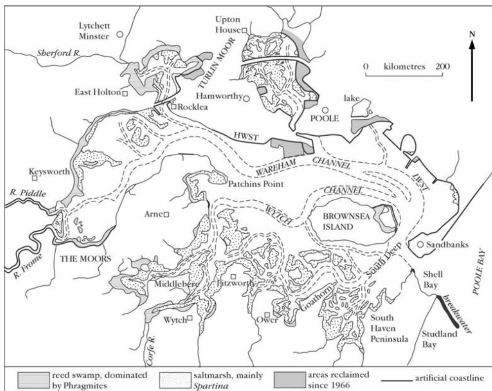
Figure 10.2: Marshes in Poole Harbour, Dorset. Common cord-grass Spartina anglica saltmarsh has developed here since 1899, and this is backed in the upper reaches by Phragmites australis reedswamp, where salinity is reduced by freshwater inflow. Saltmarsh has been reclaimed by embanking, especially near the northern urbanized fringes. (After Bird, 1984, p. 214; based on original map by V.J. May, updated to 2000)
