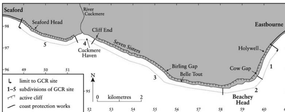
Figure 4.25: Sketch map of the Beachy Head to Seaford Head GCR site, showing the five subdivisions of the site as described in the text.
