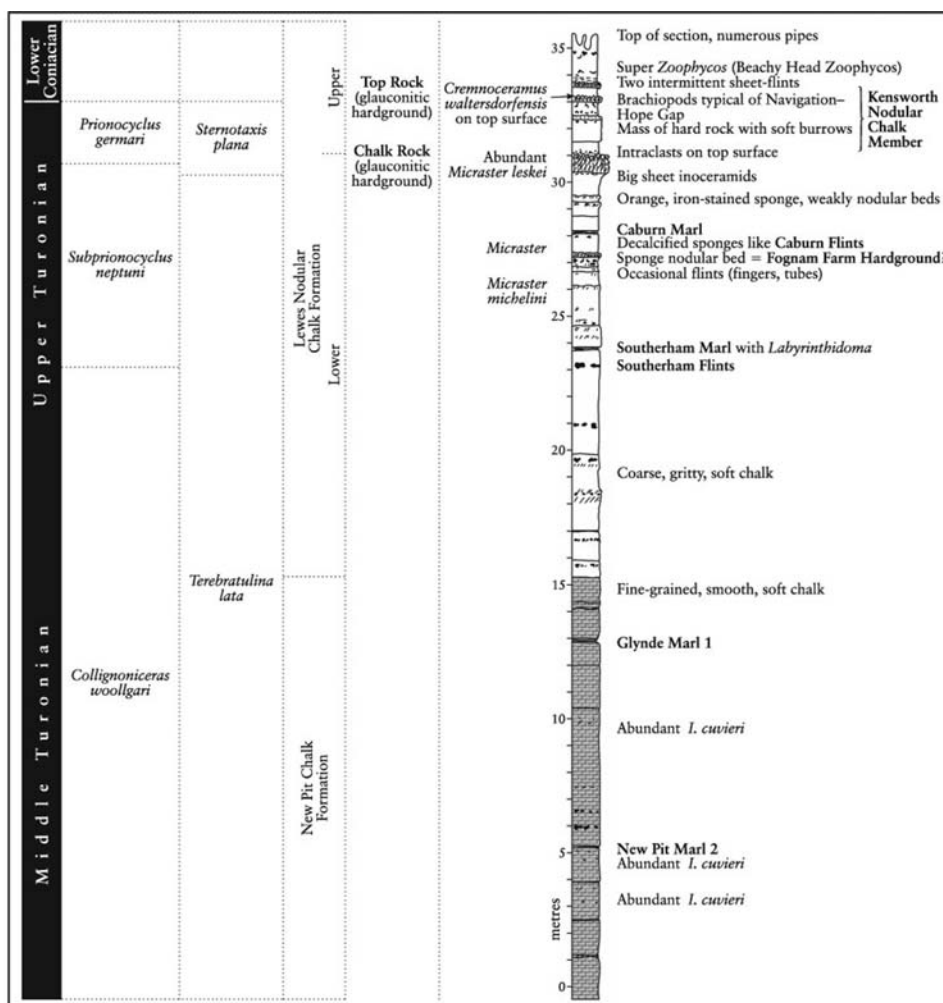
Figure 4.21: The Chalk succession at Kensworth Chalk Pit, where the inter-basinal Turonian marker marl seams are present and the northward change in development of the Chalk Rock and Top Rock is illustrated.
