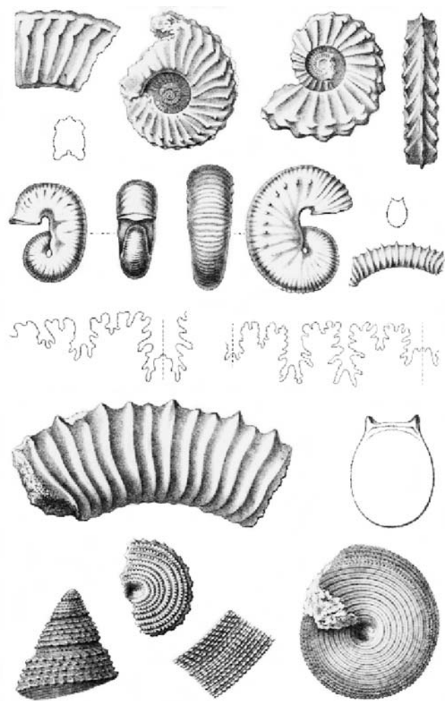
Figure 2.11: Upper Turonian mollusca of the Chalk Rock (from Woods, 1896; see also Wright, 1979). (A, B, D) Subprionocyclus neptuni . (C) Subprionocyclus branneri . (E, F, G) Scaphites geinitzii . (H, I, J) Allocioceras angustum . (K, L) Turcica? schlueteri . (M, N) Bathrotomaria perspectiva . (O, P) Metaptychoceras smithi . (Q, R, S) Hyphantoceras reussianum . (T, U, V) Eubostrychoceras saxonicum . (W, X) Sciponoceras bohemicum .
