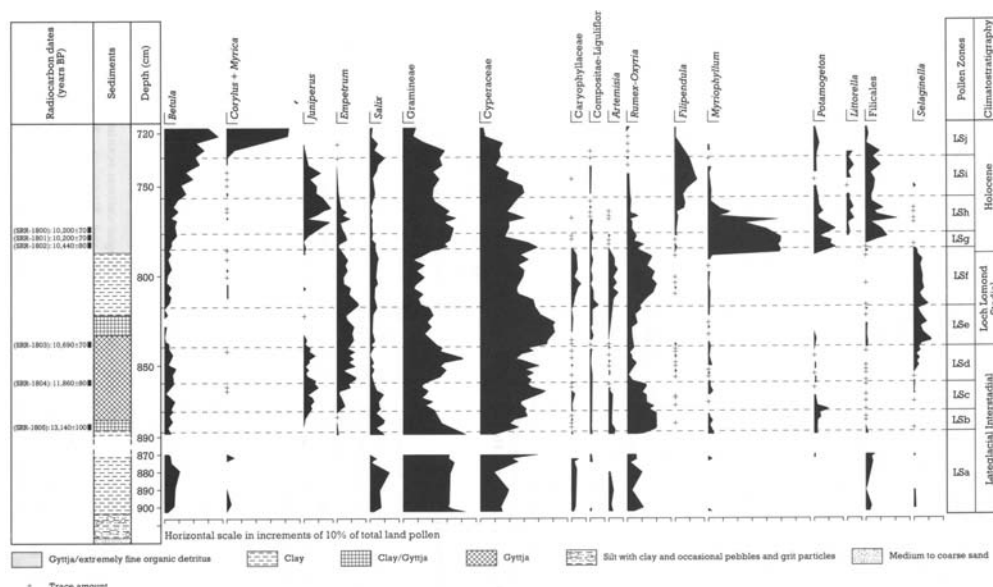
Figure 11.15: Loch an t-Suidhe: relative pollen diagram showing selected taxa as percentages of total land pollen (from Lowe and Walker, 1986a).
