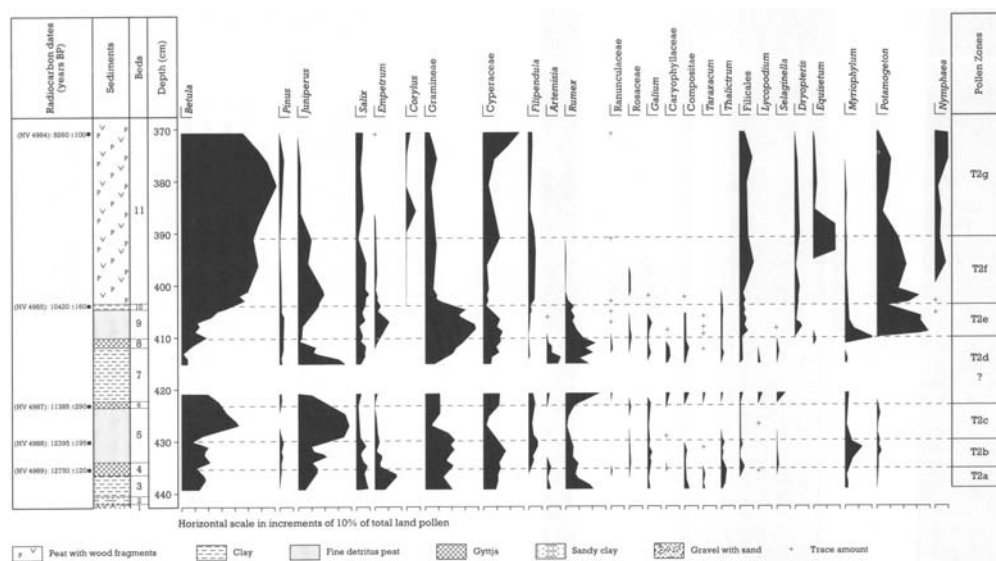
Figure 13.13: Tynaspirit: relative pollen diagram showing selected taxa as percentages of total land pollen (from Lowe, 1978).
