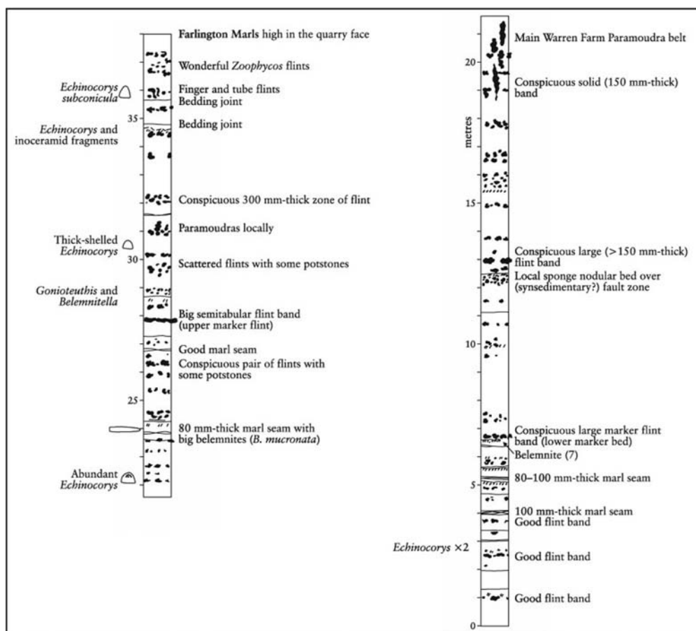
Figure 3.81: The Campanian Chalk succession at Warren Farm Chalk Pit, Portsdown. A vital link with Downend Chalk Pit.
