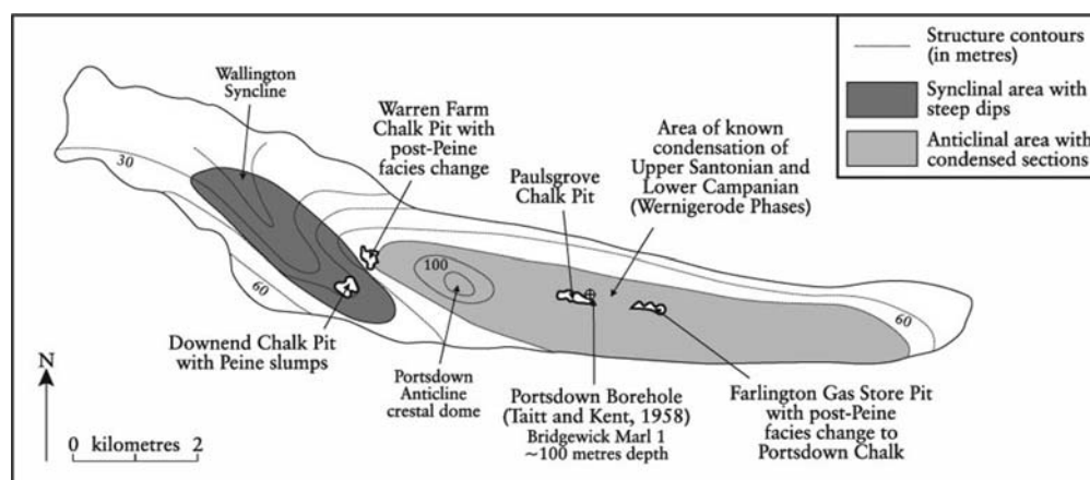
Figure 3.79: Structure contours on the Chalk of Portsdown, showing the shape of the Portsdown Anticline and Wallington Syncline. Peine phase tecto-sedimentary structures are present at Downend Chalk Pit and Warren Farm Chalk Pit, close to the crest and western flank of the structure. (From Mortimore and Pomerol, 1997.)
