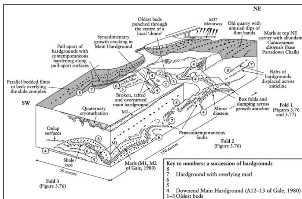
Figure 3.75: Sketch of the geology of the Culver Chalk Formation formerly exposed in Downend Chalk Pit, Portsdown. Hardgrounds, growth structures and slumps are interpreted as resulting from latest Early Campanian Peine Phase tectonic uplift. (From Mortimore, 1979, 1983; and Gale, 1980).
