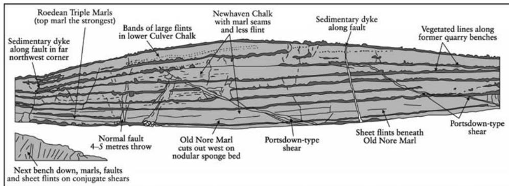
Figure 3.82: Paulsgrove Chalk Pit, Portsdown, Portsmouth, Hampshire.
