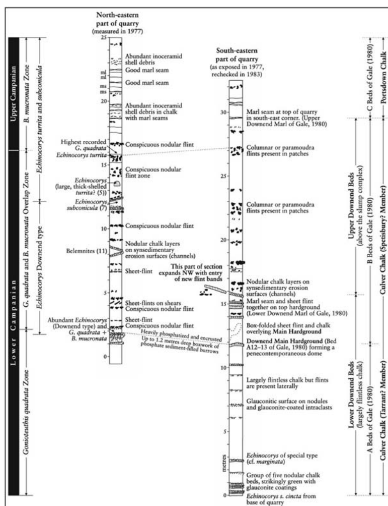
Figure 3.78: Stratigraphy of the Campanian Chalk originally exposed at Downend Chalk Pit, Portsdown. Any two sections are different as syndimentary channels and growth of penecontemporaneous slump folds create local pockets of expanded or condensed sediments. The sections shown are an attempt to illustrate the total range of the stratigraphy and the main subdivisions unravelled from the slump complex. (ms = marl seam; ml = marly laminae.)
