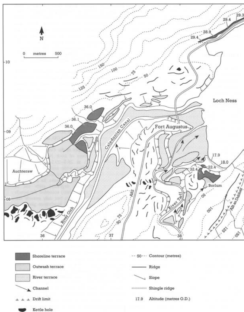
Figure 7.18: Geomorphology of the Fort Augustus area (from Firth, 1984).
