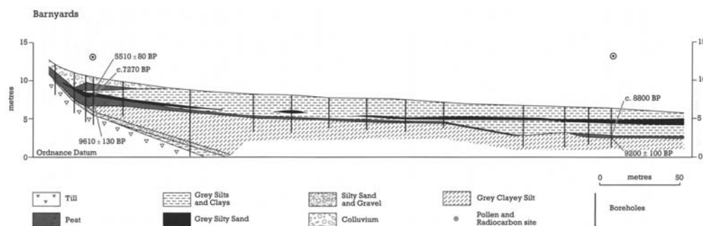
Figure 7.21: Section through the Beaully carselands at Barnyards, showing the sequence of Late Devensian and Holocene deposits (from Haggart, 1986).
