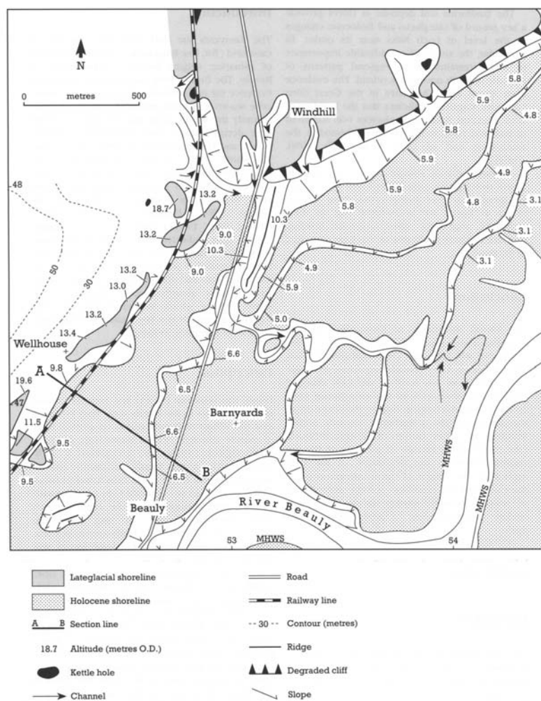
Figure 7.20: Geomorphology of the Beaully carselands (from Firth, 1984).
