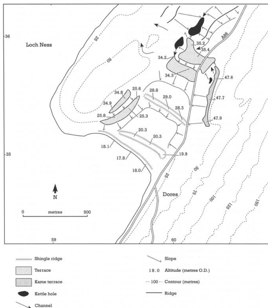
Figure 7.19: Geomorphology of the Dores area (from Firth, 1984).
