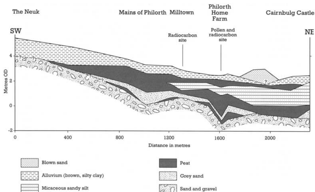
Figure 8.12: Section along the length of the Lower Philorth Valley showing the sequence of sediments (from Smith et al. , 1982).
