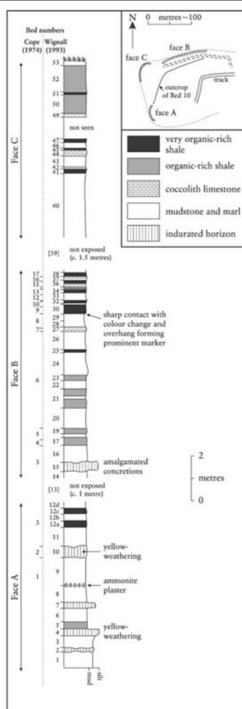
Figure 4.27: Composite graphic log of the section at Golden Hill Pit (after Wignall, 1993, fig. 3).
