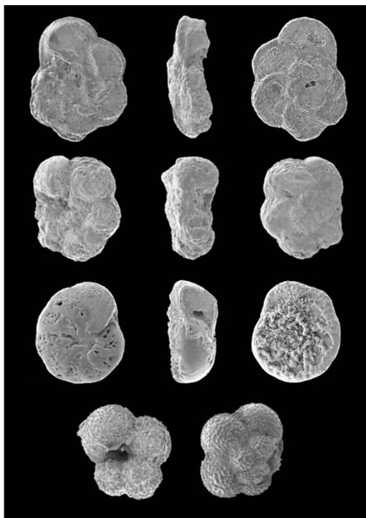
Figure 2.41: Turonian and Coniacian foraminifera (see page 77 for details).
