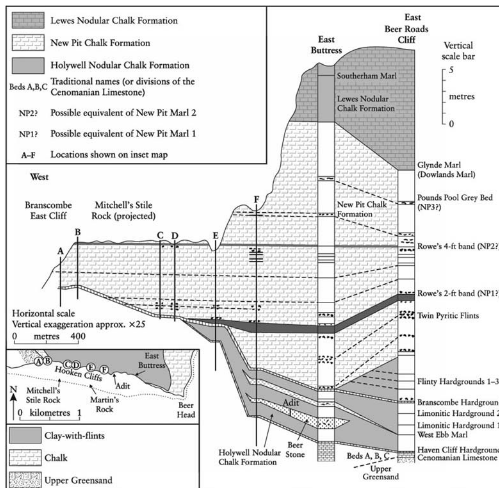
Figure 3.22: Overstep of the Upper Cretaceous Chalk (New Pit Chalk Formation) onto the Albian Upper Greensand. Lateral variation shows the Beer Stone as a lensoid sedimentary body within the Hooken–Wilmington Trough and the complete loss of the Holywell Chalk and lower New Pit Chalk traced westwards within the Hooken Cliff GCR site.
