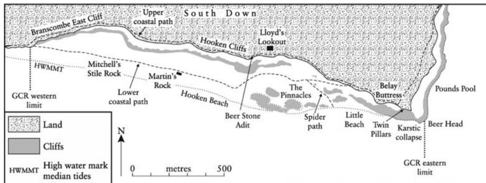
Figure 3.20: The Hooken Cliff GCR site, detailed locality map.
