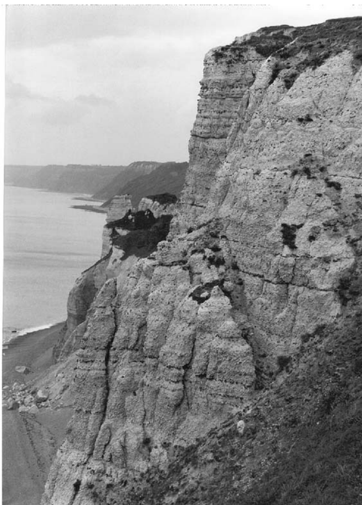
Figure 3.24: Two sections west of Beer Head, Hooken Cliff, south-east Devon, showing the entire undisturbed Upper Cretaceous succession exposed in the south-east Devon faulted outliers. (a) West side of Beer Head above Little Beach. (b) Section on 'Belay Bluff' above Beer Head. (AKF = Annis' Knob Flint (Rowe's 'strong nodular flint line'); BHLF = Beer Head Limestone Formation; BPF and BWF = Bopeep Flints and Bridgewick Flints; HNCf = Holywell Nodular Chalk Formation; NM = Navigation Marl, (Rowe's 'marl in M.c.t. '); NP1, NP2 = New Pit Marls 1 and 2; SF = sheet-flint (Rowe's 'Tabular at Base M.c.t.').) (Photos: R.N. Mortimore.)
