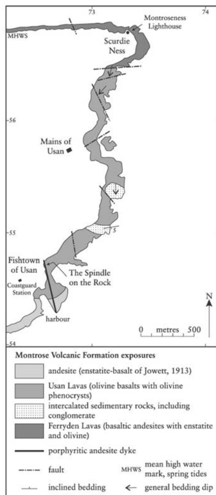
Figure 9.21: Map of coastal exposures of Montrose Volcanic Formation between Scurdie Ness and Usan Harbour, adapted from Jowett (1913).
