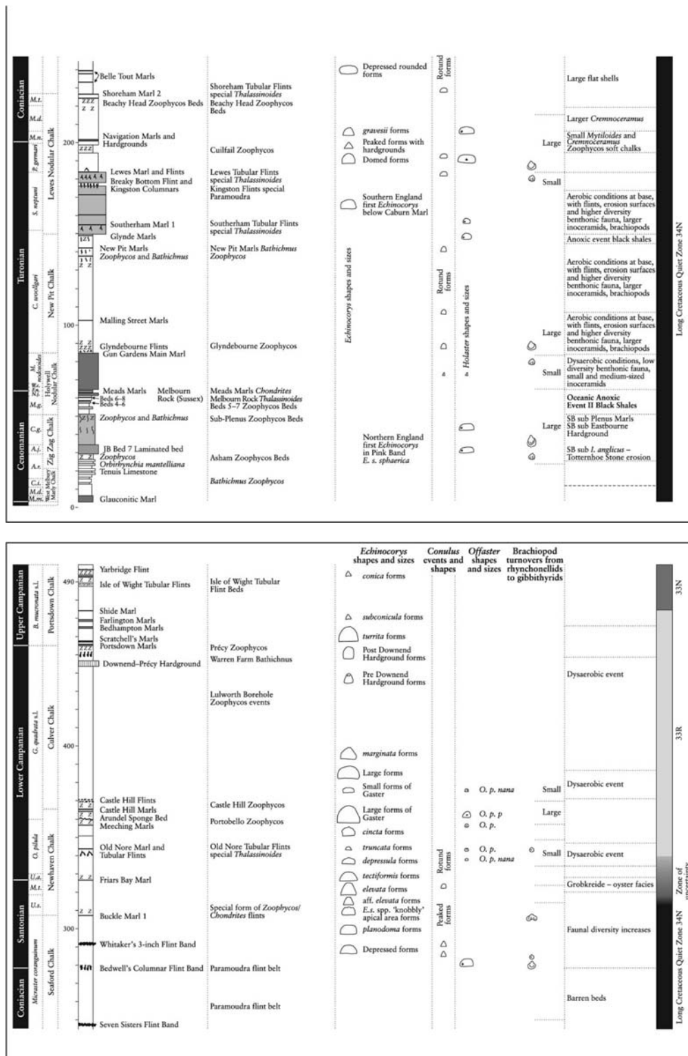
Figure 2.3: Integration of trace fossil events with shape and size changes in some key benthic fossils, and the magnetostratigraphy for the Upper Cretaceous succession in southern England. See Figure 1.5, Chapter 1, for full details of zonal fossils.
