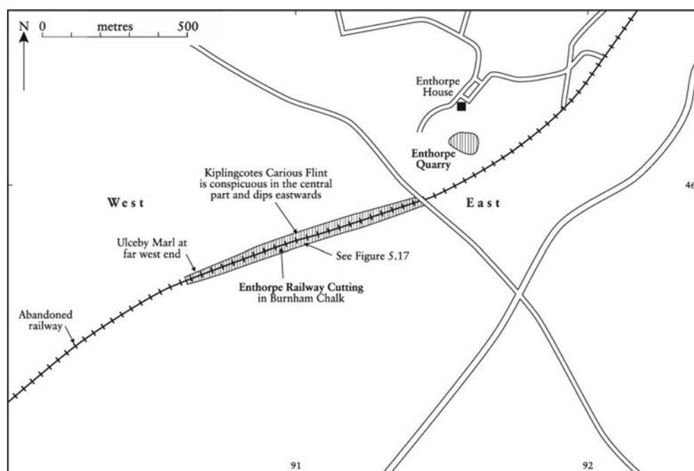
Figure 5.16: The Enthorpe Railway Cutting GCR Site, exposing the Burnham Chalk Formation from just above the Ulceby Marl to a level above the Easthorpe Tabular Flints in the Beachy Head Zoophycos Beds.
