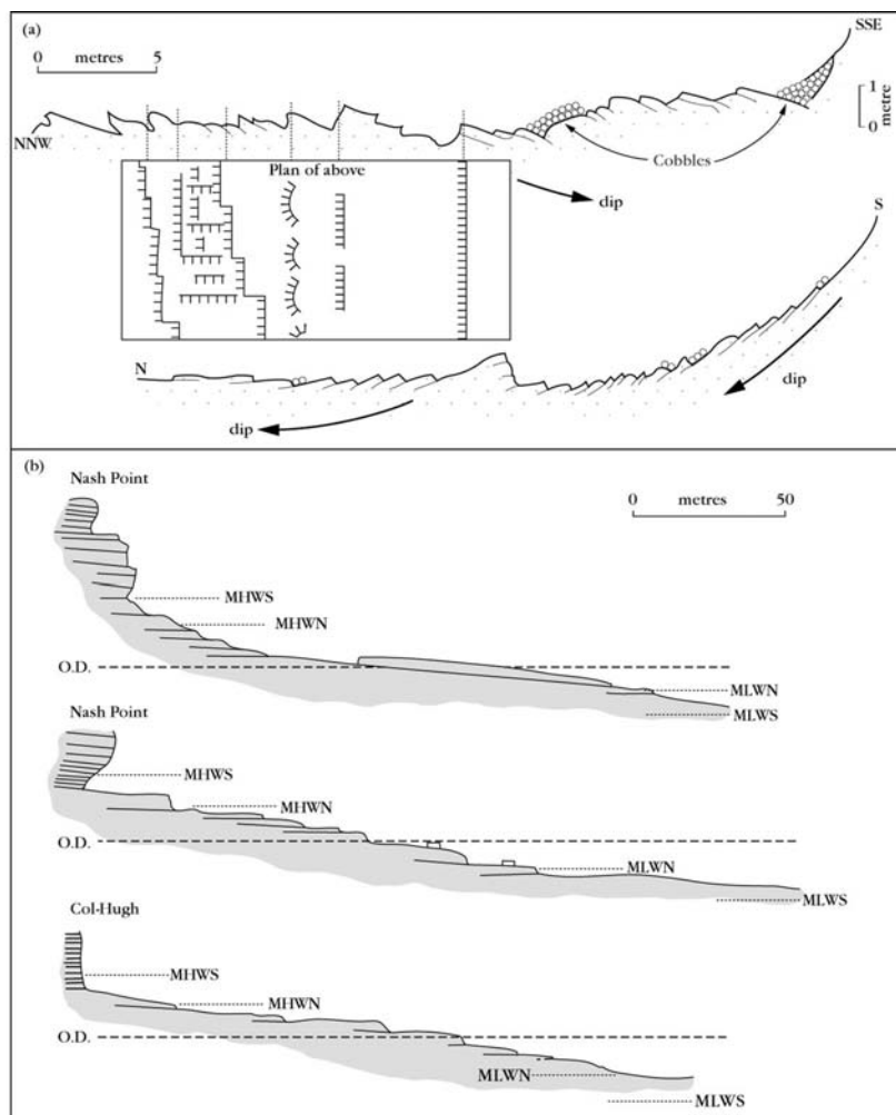
Figure 4.8: (a) Cross-sections, showing characteristic forms of the platform east of Watchet, where the dip of strata to landward or seaward strongly affects the pattern of micro-cliffs, (b) three characteristic platform profiles at Nash Point, Vale of Glamorgan (see GCR site report in the present chapter) where dip of strata is more uniform than at Watchet. Mean high- and low-water spring tide levels (MHWS and MLWS) and mean high- and low-water neap tide levels (MHWN and MLWN) are shown. (Part (b) is after Trenhaile, 1972.)
