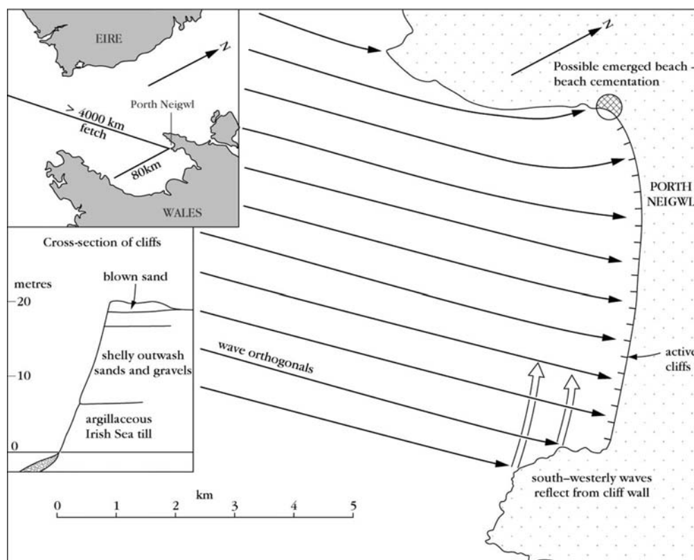
Figure 4.39: Wave refraction and reflection in Porth Neigwl. Wave orthogonals show the direction of travel of waves and are drawn at right angles to the wave crest. Open arrows are also orthogonals for reflected waves.
