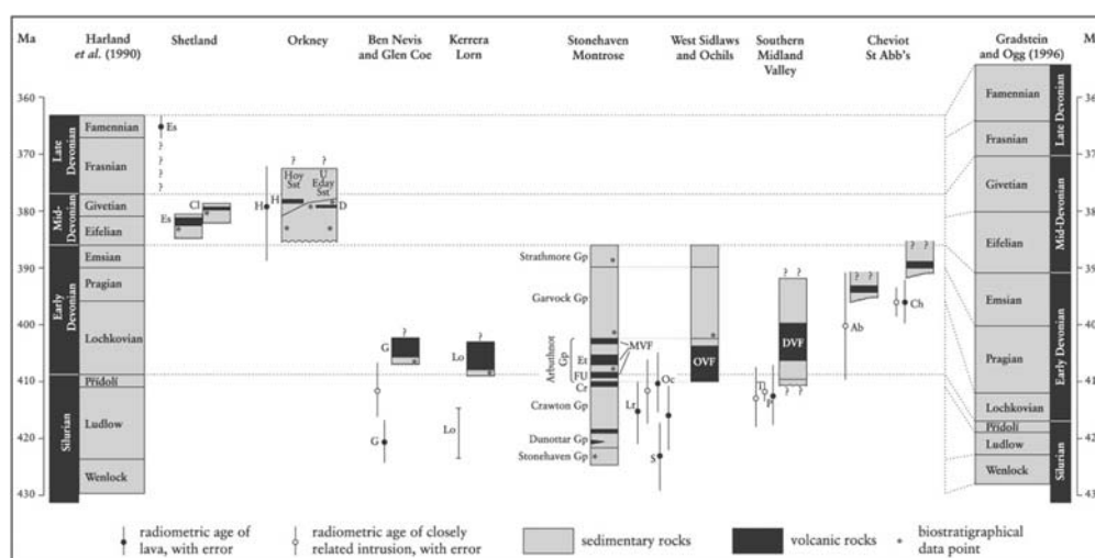
Figure 9.2: Stratigraphical relationships and ages of late-Silurian to Mid-Devonian age volcanic rocks of northern Britain. Biostratigraphical ages (where known) are given precedence and are plotted relative to the time-scale of Harland et al. (1990) (on the left). Note the consistent discrepancies between the biostratigraphical ages and the radiometric ages, which are not present if the time-scale of Gradstein and Ogg (1996) (on the right) is used. Where there is no biostratigraphical control (i.e. Southern Midland Valley, St Abb's and Cheviot), the volcanic sequences are projected from the radiometric dates. For example Cheviot at 396 Ma is early Emsian on the Gradstein and Ogg timescale, so it is plotted in the early Emsian position on the Harland et al. time scale. Ab, St Abb's; Ch, Cheviot; Cl, Clousta; Cr, Crawton; D, Deerness; DVF, Duneaton Volcanic Formation; Es, Eshaness, Papa Stour and Melby; Et, Ethie; FU, Ferryden and Usan; G, Glen Coe; H, Hoy; Lo, Lorn; Lt, Lintrathen; MVF, Montrose Volcanic Formation; Oc, Ochil Hills; OVF, Ochil Volcanic Formation; P, Pentland Hills; S, Sidlaw Hills; T, Tinto.
