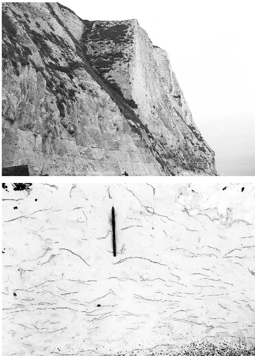
Figure 3.10: Chalk adjacent to St Margaret's Bay, Dover. (a) South side of St Margaret's Bay beyond the South Foreland, showing the Cuilfail Zoophycos in the topmost Turonian strata. (b) North side of St Margaret's Bay, showing the topmost Lewes Nodular Chalk and basal Seaford Chalk formations. (Photos: R.N. Mortimore.)
