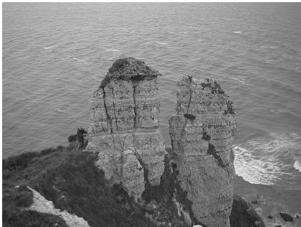
Figure 3.11: Hooken Cliff and the Twin Pillars at Beer Head; pinnacles of Lewes Nodular Chalk Formation exposing the succession from below the Annis' Knob Flint, through the Lewes Marl and Navigation Marl to a horizon around the Hope Gap Hardground equivalent. The first sheet-flints were used by Rowe (1903) for correlation. (Photo: R.N. Mortimore.)
