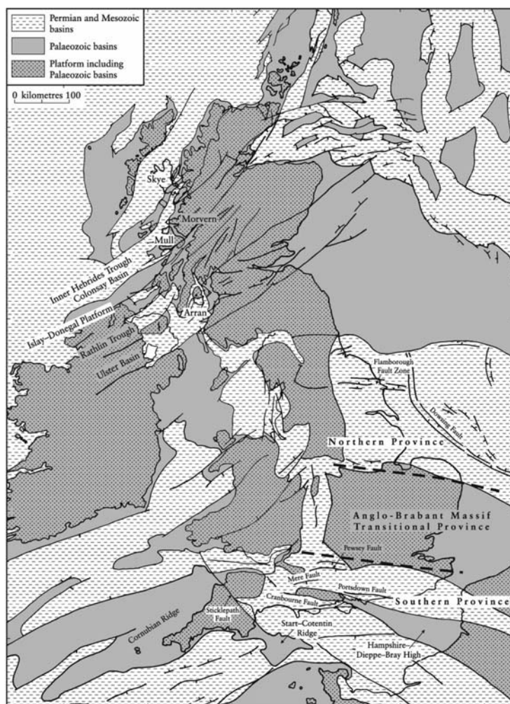
Figure 1.8: Broad structural features affecting sedimentation of the Upper Cretaceous deposits in the British Isles. (Based on British Geological Survey 1:1 000 000 maps of the Geology of the UK, Ireland and Continental Shelf, North and South Sheets.)
