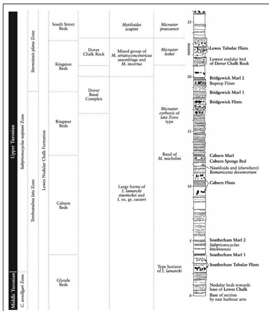
Figure 3.121: The lowest sections on Langdon Stairs including the Dover Chalk Rock and Basal Complex. (Based on Mortimore, 1997.)
