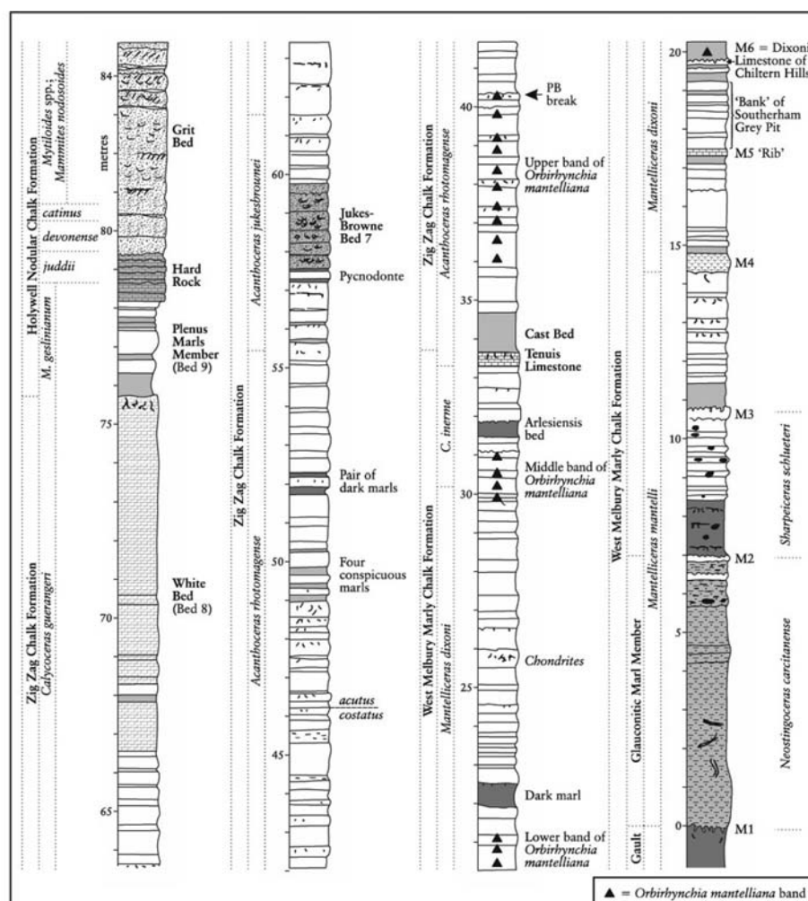
Figure 3.119: The Grey Chalk Subgroup type section at Folkestone, Abbot's Cliff, showing key litho- and biostratigraphy. (Modified from Gale in Jenkyns et al. , 1994: and Mortimore, 1997.) The black symbols in the schlueteri Subzone represent spongy nodules.
