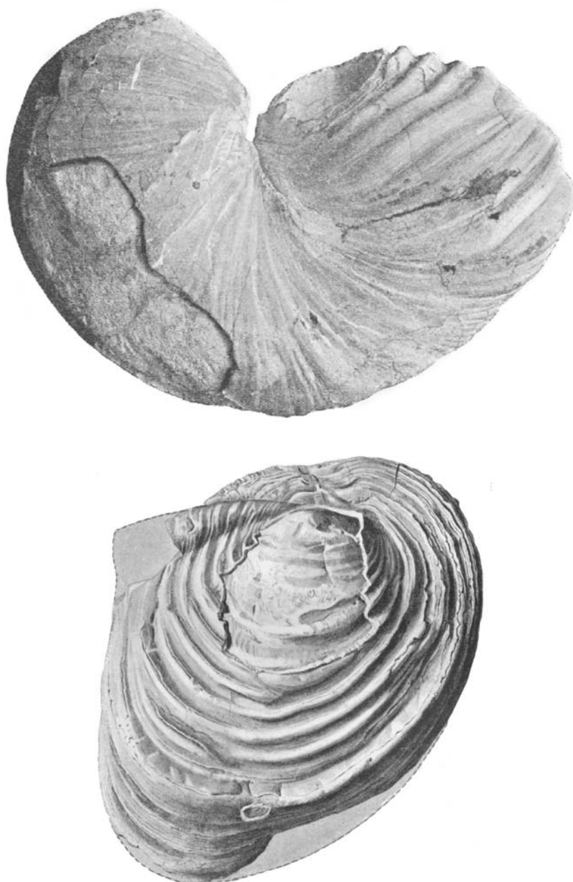
Figure 2.20: Lower and Middle Coniacian inoceramid bivalves. (A) Cremnoceramus crassus crassus typical of Beeding to Light Point beds, Lewes Nodular Chalk (from Walaszczyk and Wood, 1999b, pl. 17, fig. 2). (B) Fragments of Platyceramus sp. shell typical of the Belle Tout Beds, Seaford Chalk Formation (from De Mercy, 1877). (C–E) Volviceramus aff. involutus ; (C, D) typical of Belle Tout Beds, Seaford Chalk Formation (from Woods, 1912, text-figs 93, 90); (E) typical cap valve in Belle Tout Beds, Seaford Chalk Formation, common 1.8–2 m below the Seven Sisters Flint Band (from Woods, 1912, text-fig. 94). Scale bar applies to all specimens.
