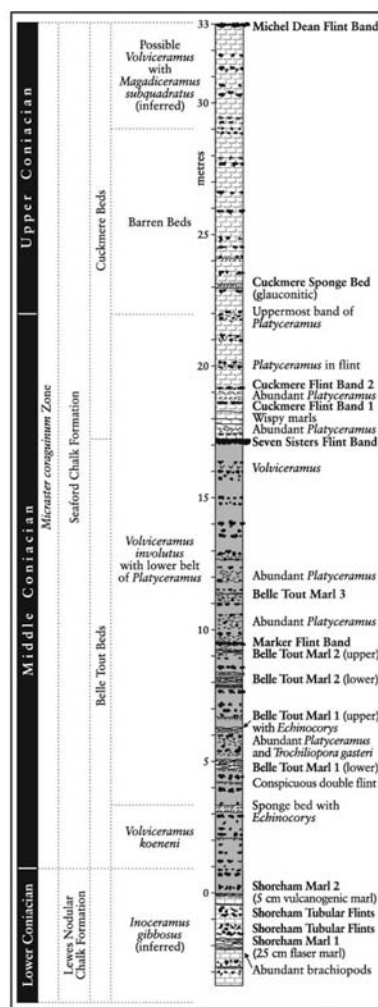
Figure 3.98: Topmost Lewes Nodular Chalk and lower part of the Seaford Chalk Formation, Cuckmere to Seaford GCR site.
