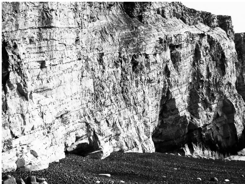
Figure 3.104: Seaford Head, Newhaven Chalk Formation, Lower Campanian Offaster pilula Zone. (BSB = Bastion Steps Beds; MB = Meeching Beds; ONB = Old Nore Beds; PB = Peacehaven Beds.) (Photo: R. N. Mortimore.)
