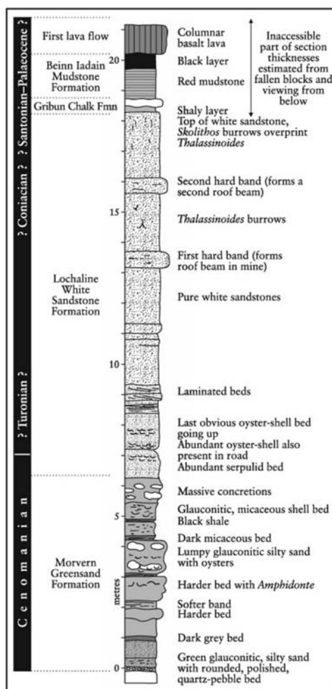
Figure 6.32: The Upper Cretaceous deposits of the Lochaline Mine Adit section, Lochaline, Morvern. The Gribun Chalk Formation probably incorporates the Clach Alasdair Conglomerate and lignites.
