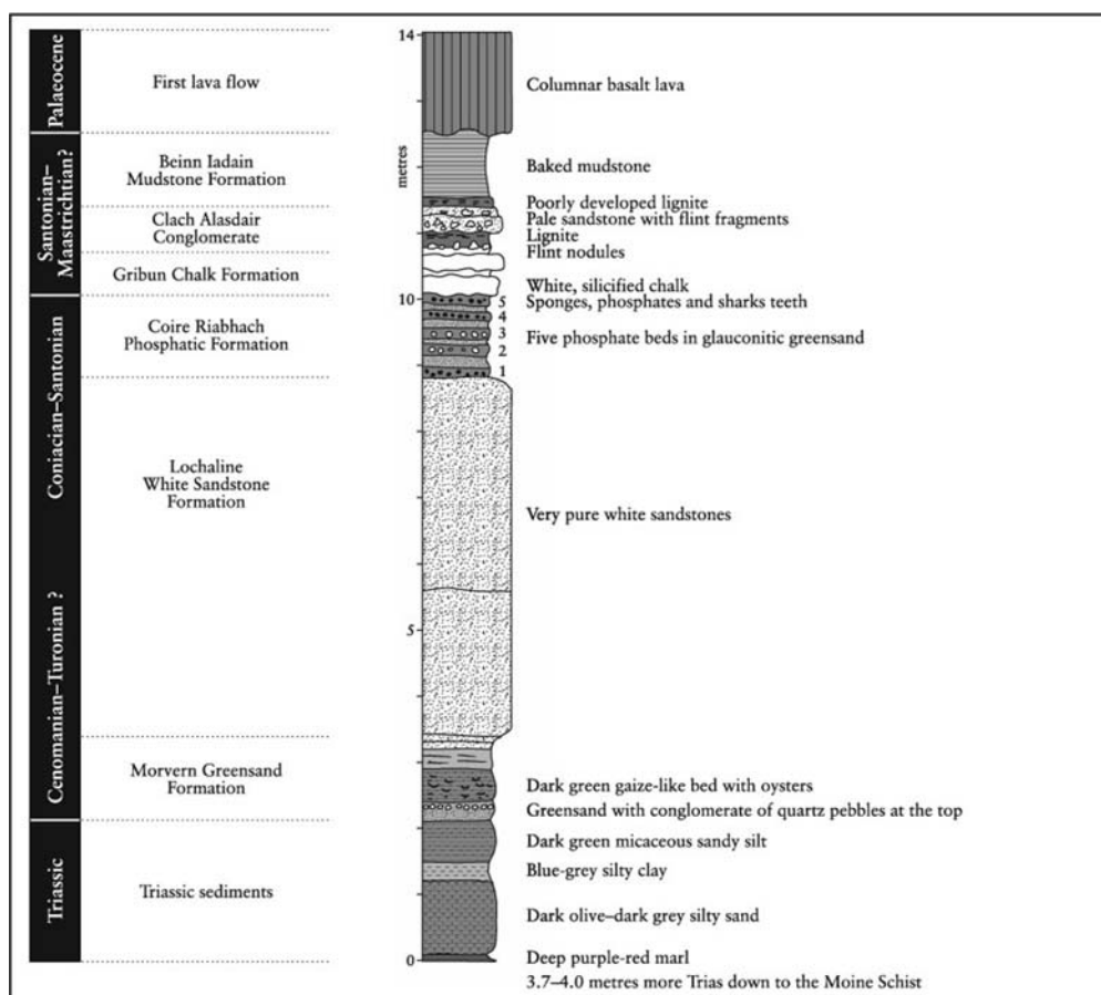
Figure 6.31: The stratigraphy of the Coire Riabhach stream section, Beinn Iadain, Morven. (Measured by R.N. Mortimore, 1999.)
