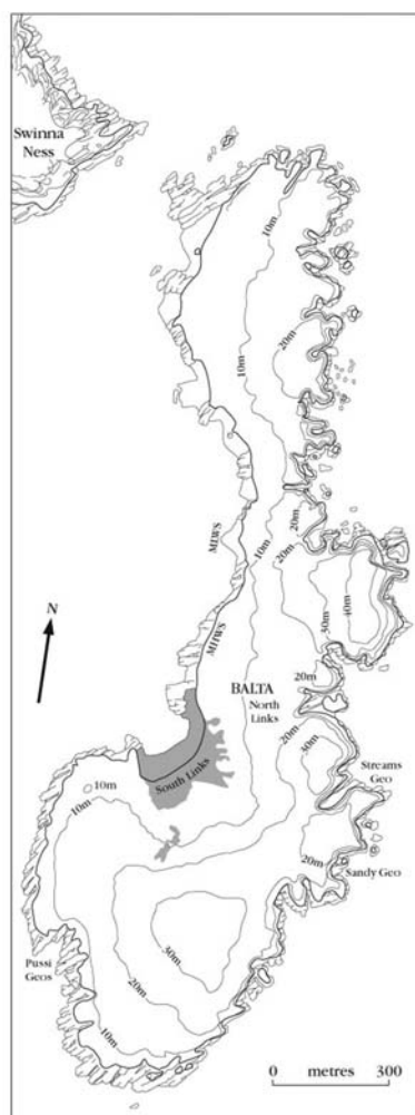
Figure 7.30: Balta Island, Unst, Shetland, is low in the west and high in the east. It is mainly rocky except where sand is blown up-slope from the beach at South Links. (After MacTaggart, 1999.)
