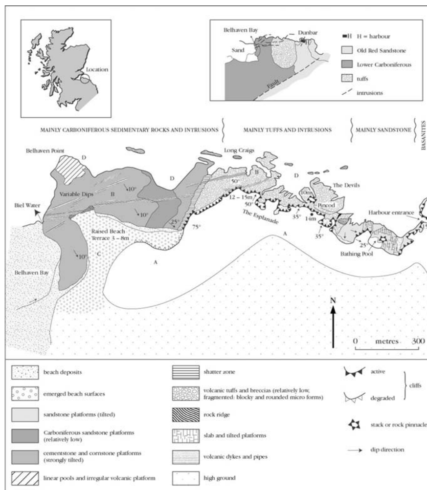
Figure 3.23: Geomorphological map and geological sketch map of the Dunbar GCR site showing a series of emerged rock shore platforms that have been eroded across a varied geology and are backed by cliffs of varying heights. Platform A lies at c. 20 m OD and is ice-moulded; Platform B is intertidal; Platform C underlies emerged Holocene beach deposits and Platform D is subtidal. (After Gordon and Sutherland, 1993.)
