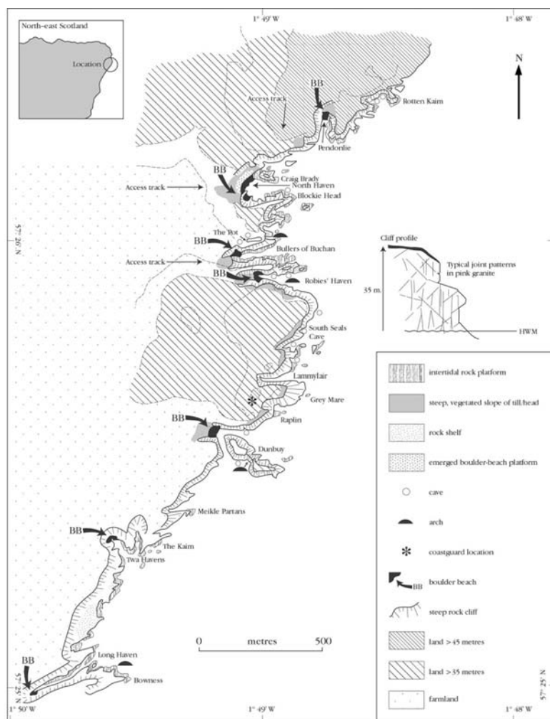
Figure 3.21: Geomorphological map of the Bullers of Buchan, north-east Scotland. The inset on the right shows the typical cliff profile relative to high-water mark (HWM). Much of the cliff tops are veneered by glacial till. (Modified from unpublished work by W. Ritchie.)
