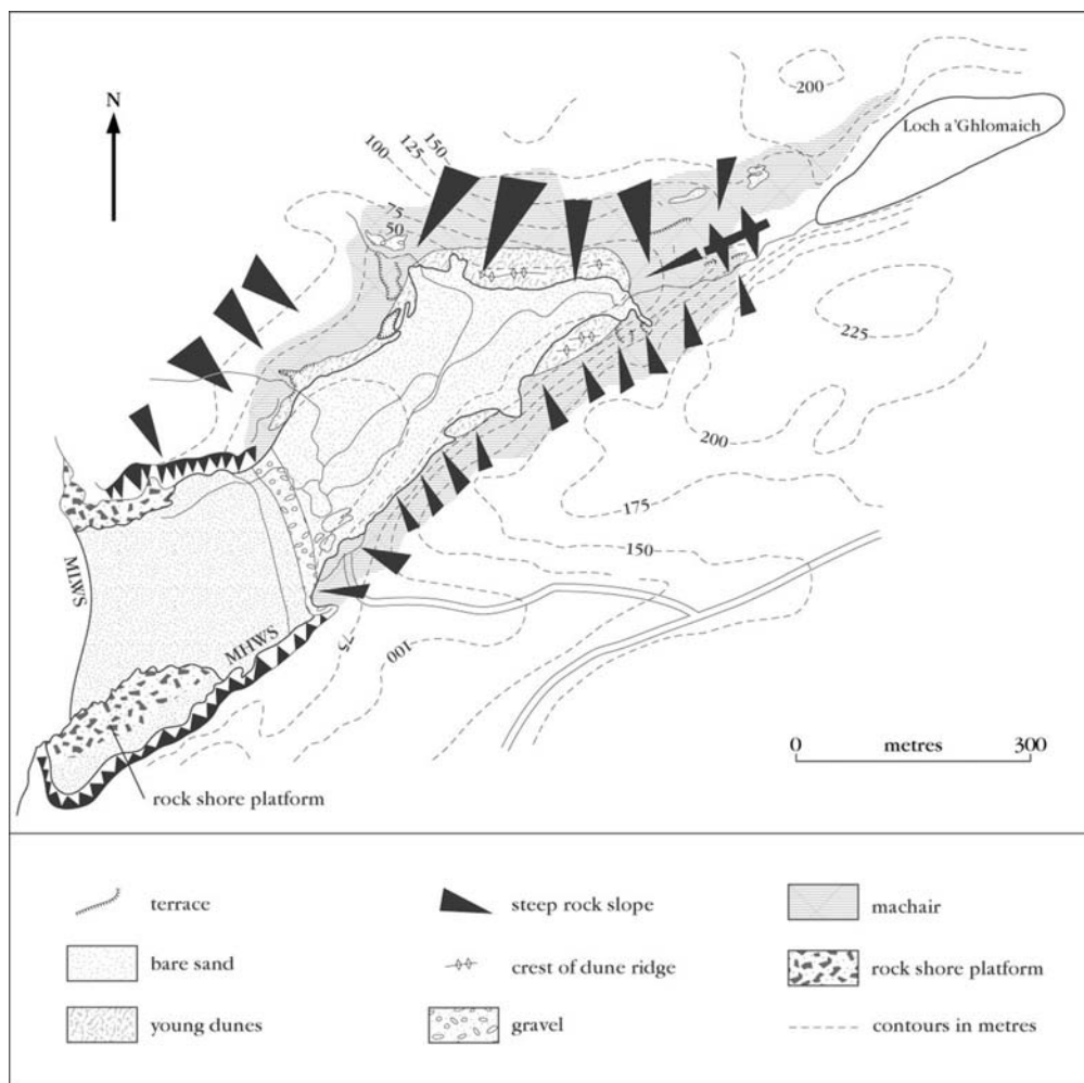
Figure 9.16: The geomorphology of the small embayment of Mangersta, Lewis. A narrow beach separates an area of low-lying sand from the sea. Mangersta is an example of a machair complex that has been eroded and deflated down to the water table. (After Ritchie and Mather, 1970b.)
