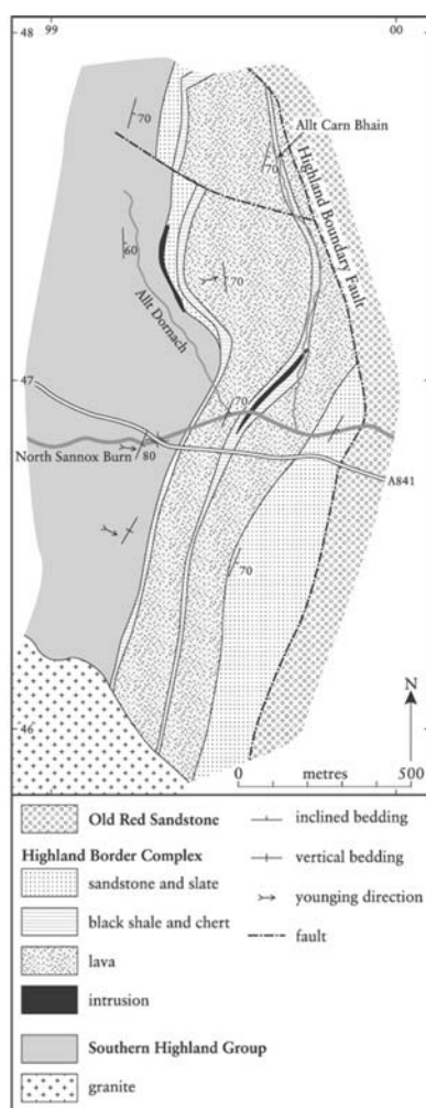
Figure 2.22: Map of the North Glen Sannox GCR site, in part after Johnson and Harris (1967) and Anderson and Pringle (1944).
