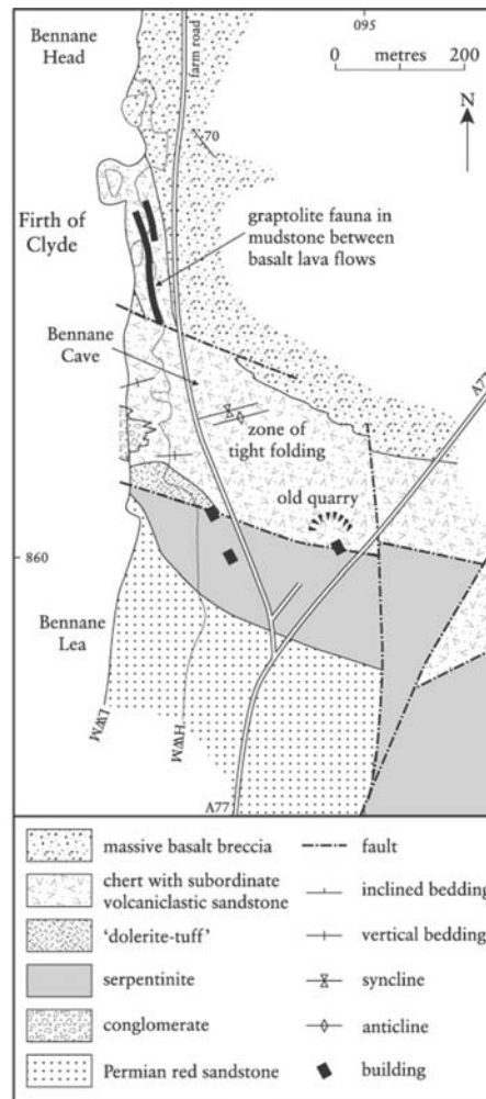
Figure 2.39: Map of the Bennane Lea area, after BGS 1:25 000 special sheet, Ballantrae (1988) and Stone and Smellie (1988).
