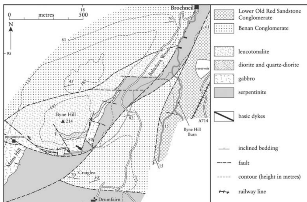
Figure 2.24: Map of the Byne Hill area (after Bloxam, 1968).
