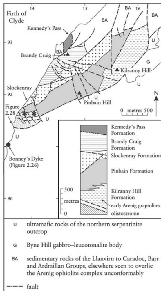
Figure 2.25: Map and stratigraphy of the Pinbain Block, the northernmost part of the Ballantrae Complex, after Bluck (1982) and Stone and Smellie (1988). * The area marked thus on the map was included within the Pinbain Formation by Bluck (1982), but is more closely related lithologically to the Kilranny Hill Formation.
