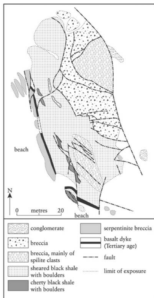
Figure 2.28: Map of the SW margin of the Pinbain olistostrome, after Bluck (1978a, 1992). See Figure 2.25 for location.
