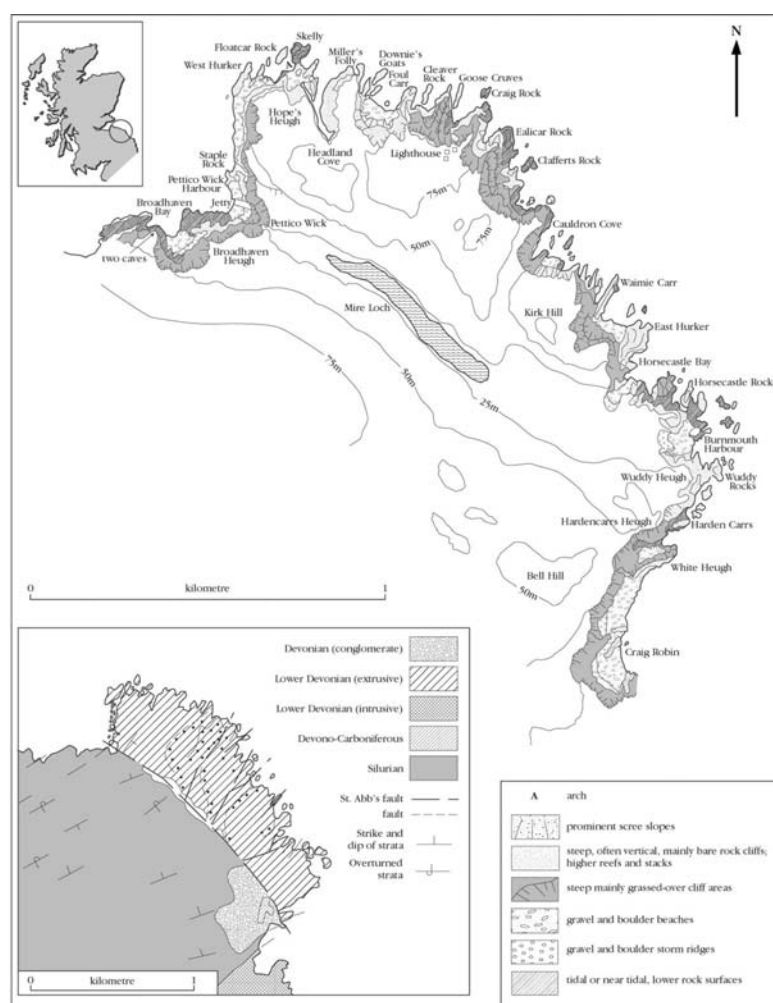
Figure 3.24: Geomorphological map and geological sketch map of St Abb's Head showing the heavily indented nature of the coast resulting from a strong structural control. (Modified from unpublished work by W. Ritchie.)
