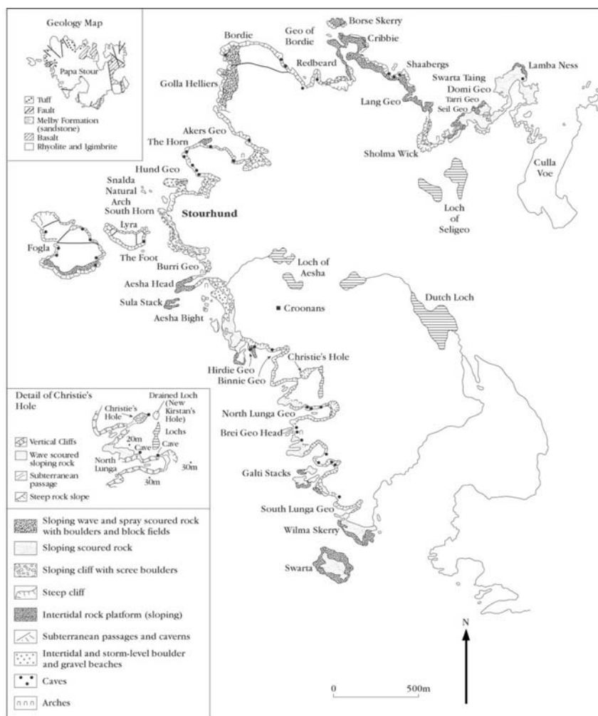
Figure 3.8: Geomorphological sketch map of Papa Stour showing extensive wave-scoured cliff-top surfaces, together with stacks, caves, arches and geos. For general location, see Figure 3.1. (Modified from unpublished work by W. Ritchie.)
