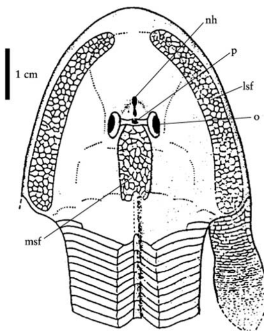
Figure 3.15: Hemicyclaspis munchisoni Lankester, detail of the dorsal surface of the headshield: p, pineal foramen; o, orbits; nh, nasal hypophysis; lsf, lateral sensory field; msf, median sensory field (after Stensiö, 1932).
