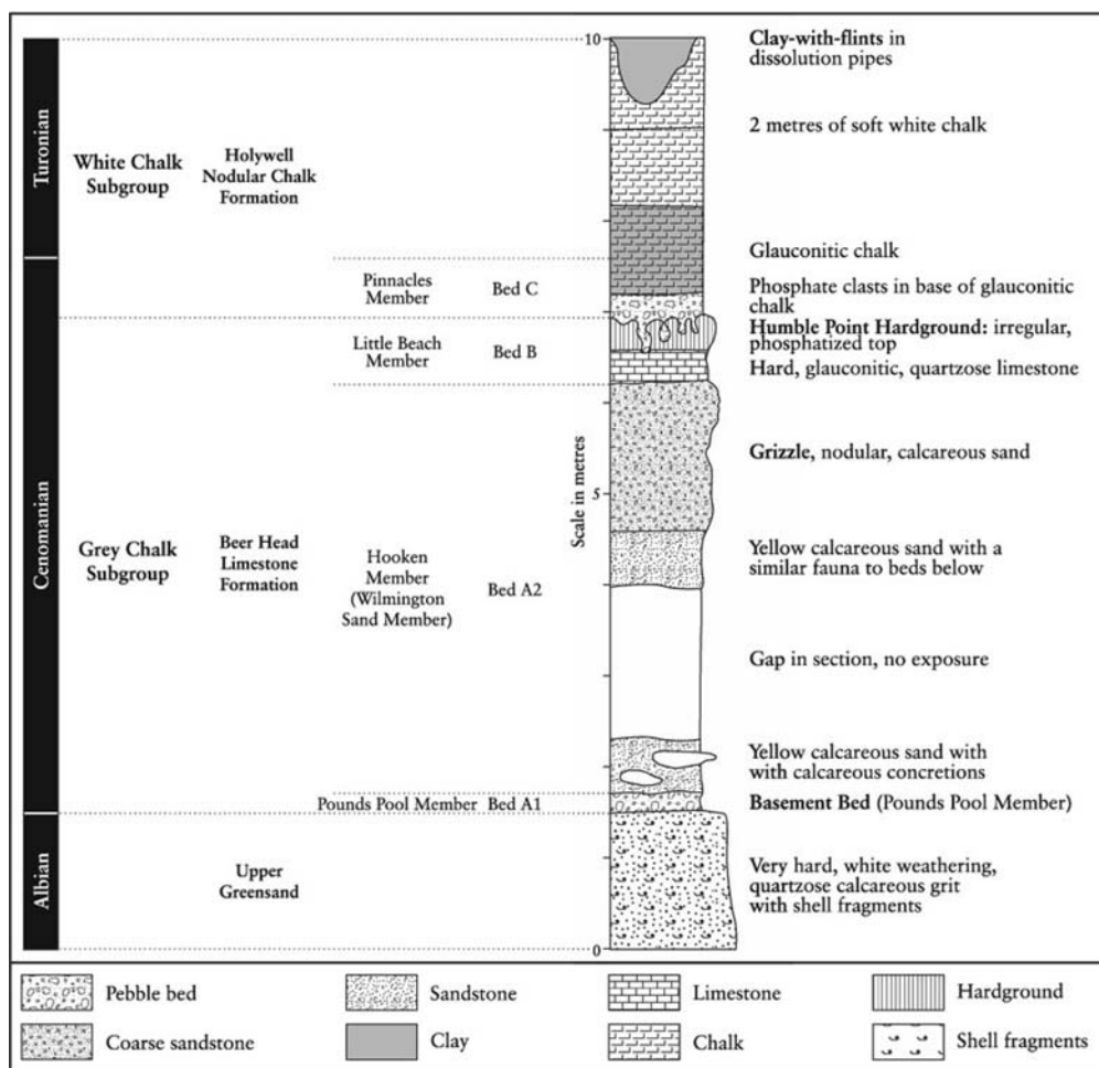
Figure 3.28: The former section at Reeds Farm Pit, Wilmington, south-east Devon (also known as 'Hutchins Pit' or 'Haynes Lane Pit').
