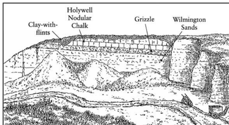
Figure 3.29: Sketch of Reeds Farm Pit, Wilmington, south-east Devon. (From Jukes-Browne and Hill 1903, fig. 31, p. 127.)
