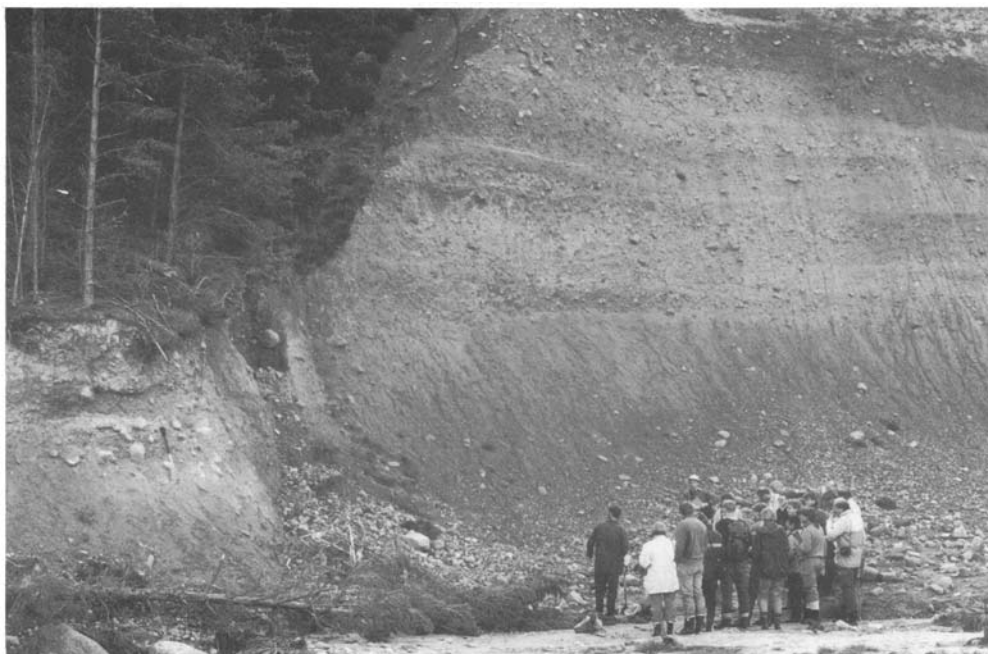
Figure 7.2: Section at Dalcharn showing the Dalcharn 'gravel formation' and the Dalcharn 'biogenic formation' (bottom left), overlain by a sequence of tills (right). (Photo: D. G. Sutherland.)
