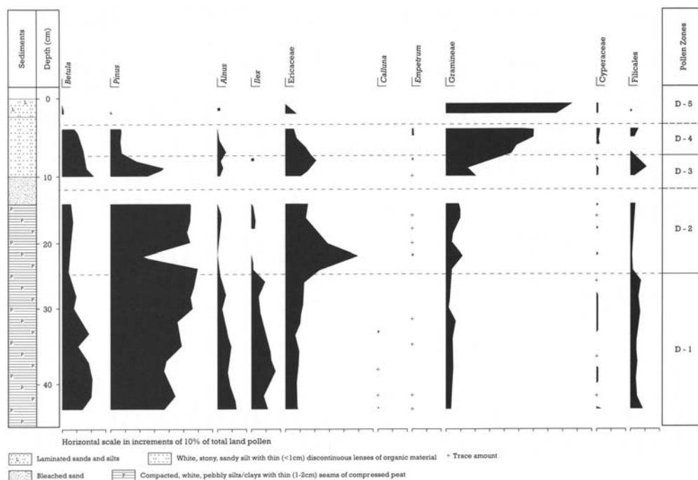
Figure 7.4: Relative pollen diagram for the Dalcharn 'biogenic formation', showing selected taxa only as percentage of total land pollen (from Walker, 1990a).
