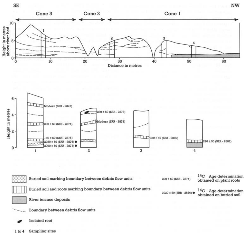
Figure 9.17: Top: surveyed section across the base of the Glen Feshie debris cones showing boundaries between individual debris-flow units. Bottom: detailed sections at sampling sites 1–4 (from Brazier and Ballantyne, 1989).
