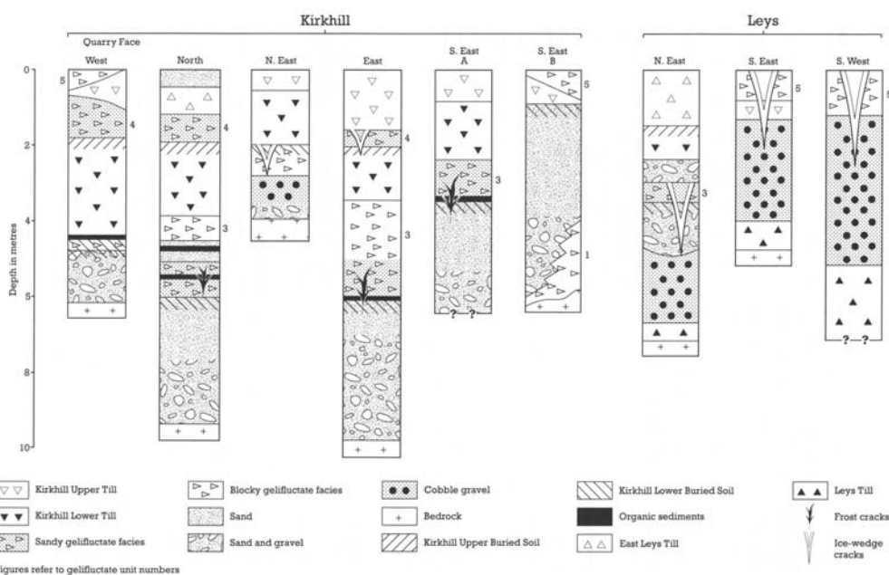
Figure 8.4: Kirkhill and Leys: lithostratigraphy.
