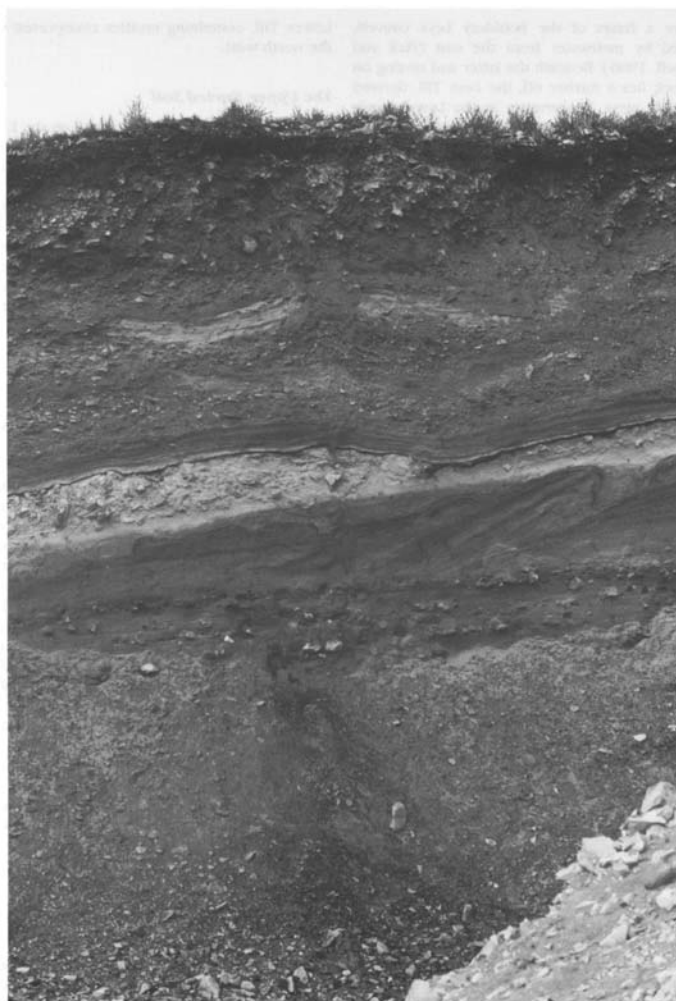
Figure 8.5: Kirkhill Quarry, south-east face B (1984). Developed in the Kirkhill Lower Sands and Gravels is the Kirkhill Lower Buried Soil, with its striking bleached horizon. The soil is truncated and overlain by laminated organic muds and sands, and then by periglacial slope deposits of Kirkhill Gelifluctate 3. These rubble layers have been partly reworked to form the Kirkhill Upper Till. The section is about 6 m high. (Photo: J. Jarvis.)
