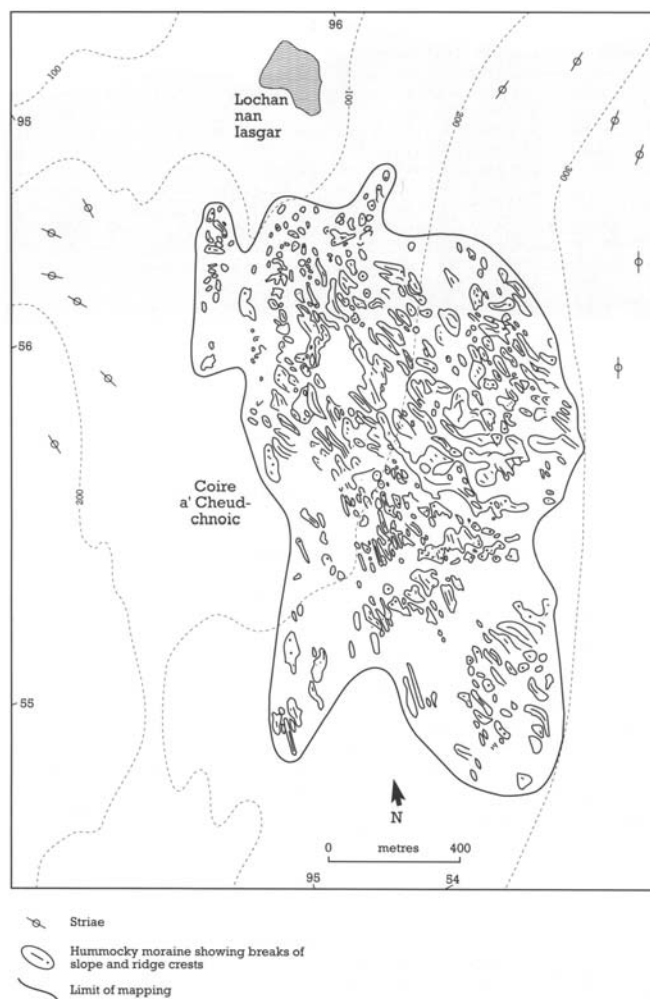
Figure 6.13: Geomorphology of Coire a'Cheud-chnoic (from Hodgson, 1987).
