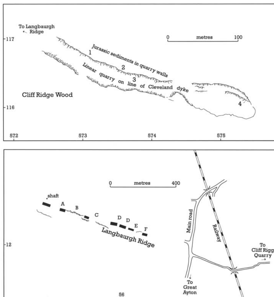
Figure 7.6: Sketch maps showing outcrops of the Cleveland Dyke near Great Ayton, North Yorkshire: (lower) Langbaugh Ridge. Localities A-F refer to points where the north margin of the dyke has been preserved. (upper) Upper part of Cliff Rigg Quarry. For explanation of localities 1-4 see text
