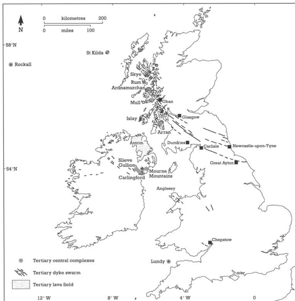
Figure 1.1: Map of the British Isles, showing the distribution of Tertiary central complexes, dyke swarms and lavas (submarine occurrences not shown). Modified from Emeleus, in Sutherland (1982, figure 29.1)
