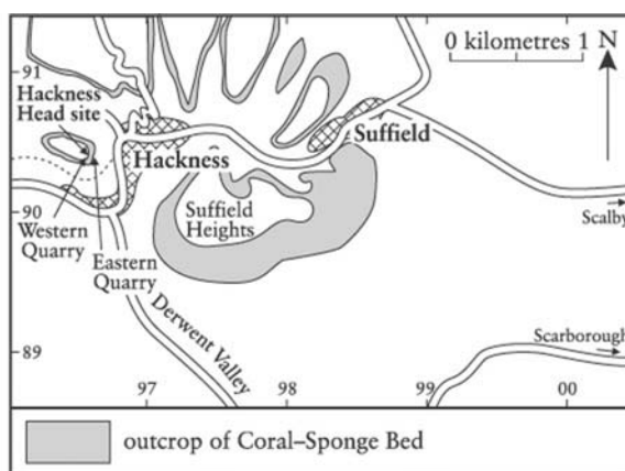
Figure 4.16: Locality map for Hackness Head showing the outcrop of the Coral-Sponge Bed (Subdivision 3). (After Wilson, 1949, fig. 43.)
