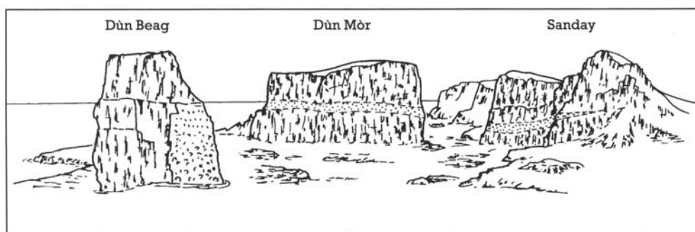
Figure 3.20: Sketch of Dùn Beag, Dùn Mòr and the cliffs of Sanday (after Harker, 1908, figure 12). Columnar basalt flows with interbedded conglomerate are seen on Dùn Mòr and the cliffs of Sanday. On Dùn Beag, lavas fill steep-sided valley eroded in conglomerate
