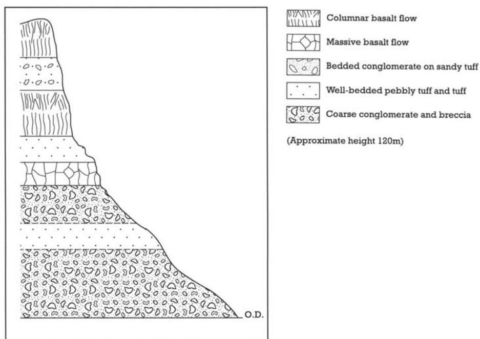
Figure 3.21: Cliff section at Compass Hill, Canna (after Harker, 1908, figure 8)
