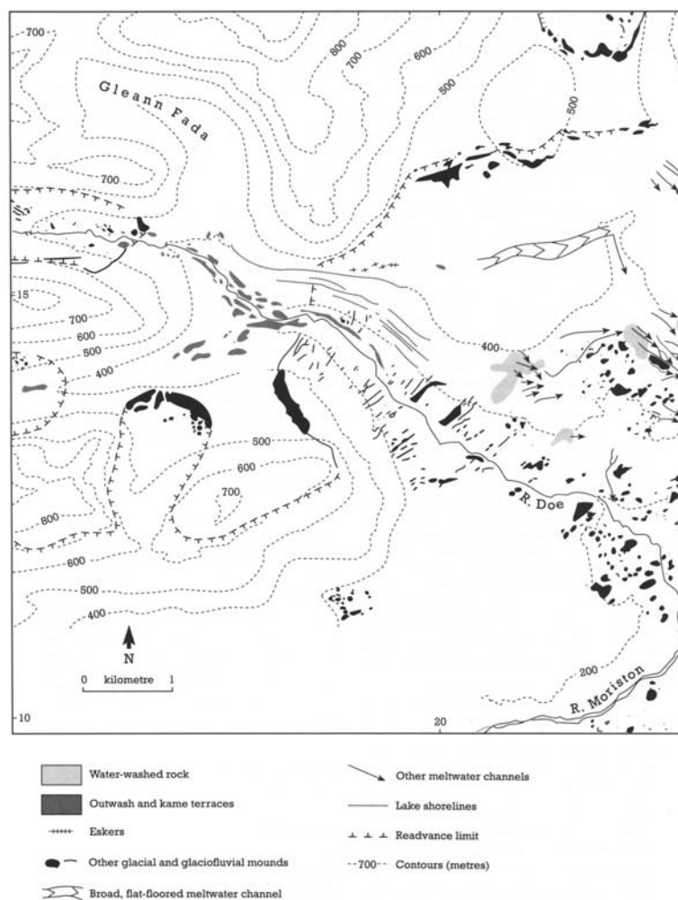
Figure 7.17: Geomorphology of Coire Dho showing landforms associated with the former ice-dammed lake (from Sissons, 1977b).
