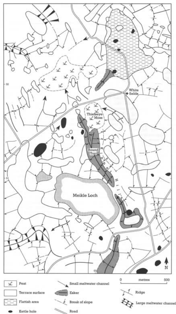
Figure 8.9: Geomorphology of the Kippet Hills (from Smith, 1984).
