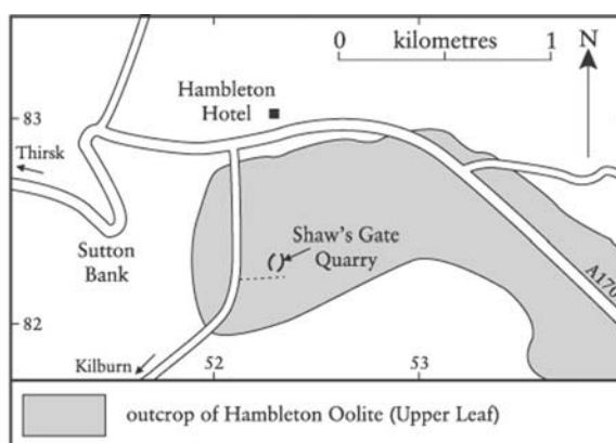
Figure 4.28: Locality map of Shaw's Gate Quarry. Outcrop of the Hambleton Oolite from BGS Sheet 52 (Thirsk) (1992).
